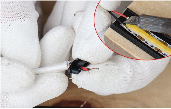
step7 - Melt the solder joint of the LED strip, remove the wire and pass it through the hole of the end cap.
