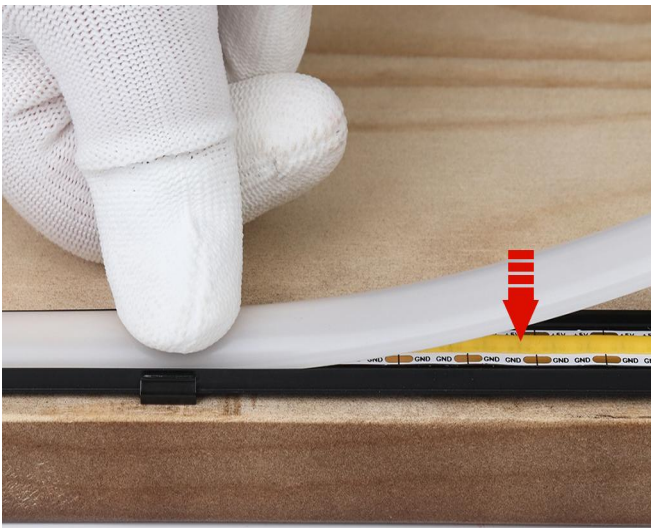
Step9 - Press the cover into the LED channel.
