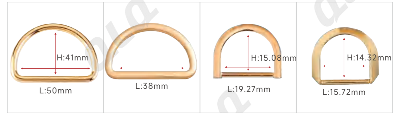
DB-10 50mm (D buckle) 2寸 (D扣)
