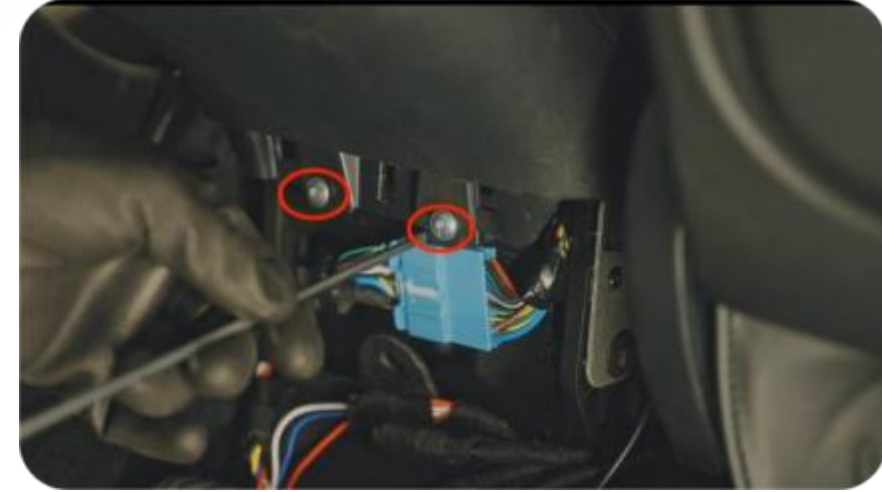
4. Unscrew the two fixing screws
