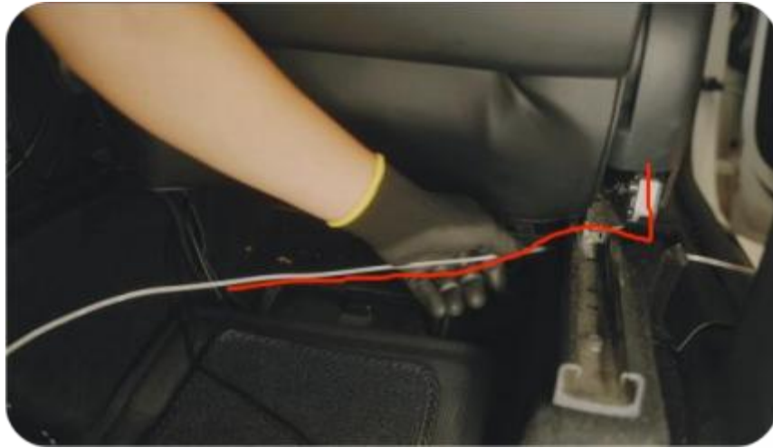
17. Thread the wiring harness under the seat from the seat adjustment position
