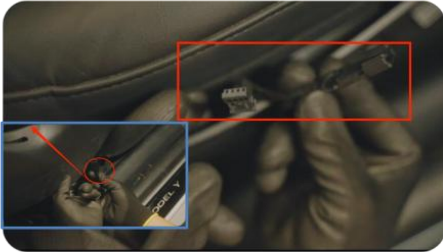
13 Thread the harness over the seat adjustment plug
