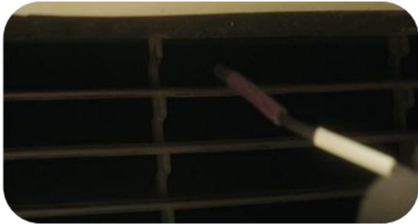
6. Pass the camera harness through the lower grille into the cabin.
