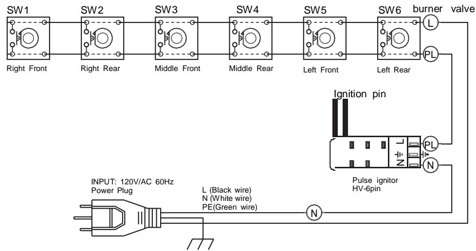
WFCT8536 Circuit Diagram
