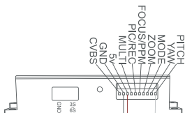
Connection Diagram (Standard Version)
